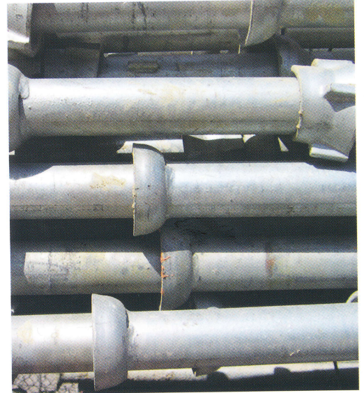
Cuplock System Scaffolding
